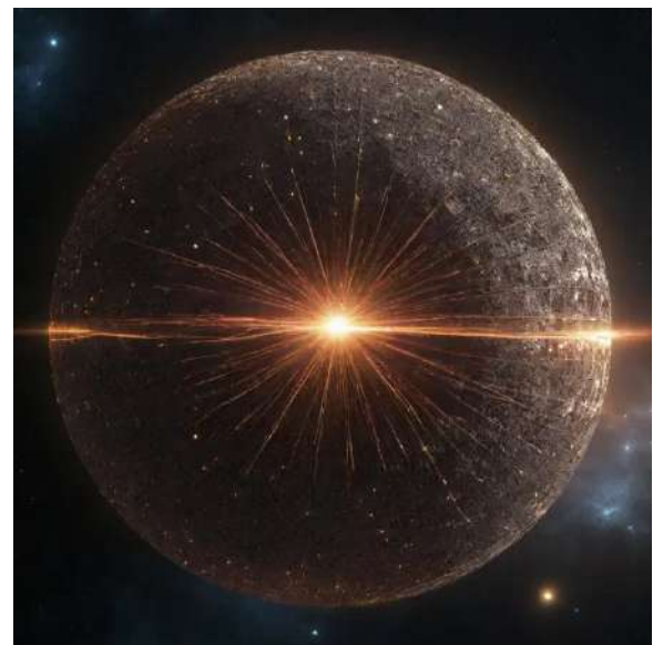
Picture 2. Dyson sphere
